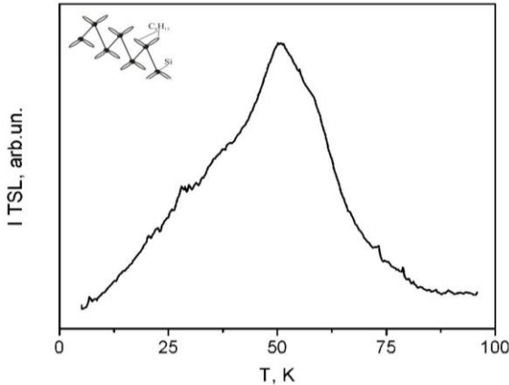
Fig. 1. Integral TSL curve of PDHS film. Inset shows structure of PDHS polymer
